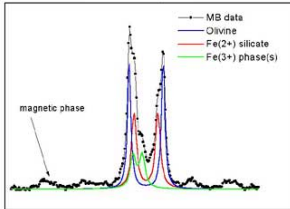
Mössbauer Spectrum on Martian Soil, Meridiani Planum, Sol 11
