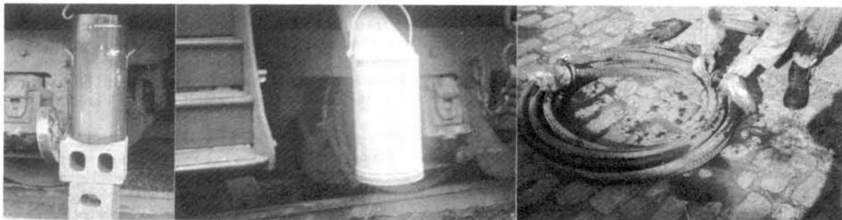
Left: Vertical soil can, properly elevated on cinder blocks with hopper outlet extending into can. Center: Proper placement of angle-spout soil can. Right: Improper storage of hose on ground illustrates value of protective plastic bags on ends.
